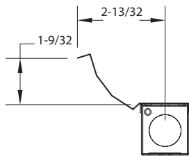
Asymmetrical Reflector
