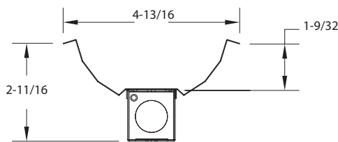
Symmetrical Reflector
